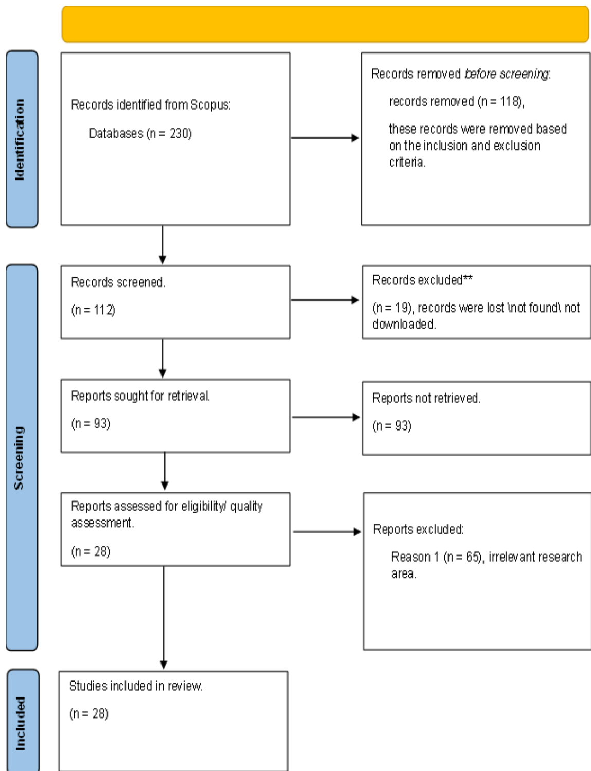
Figure 1: PRISMA framework
