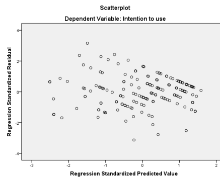
Fig. 2 Scatter plot
