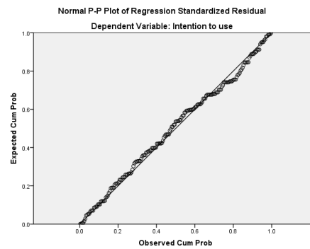
Fig. 1 Normal P-P Plot of Regression Standardized Residual
