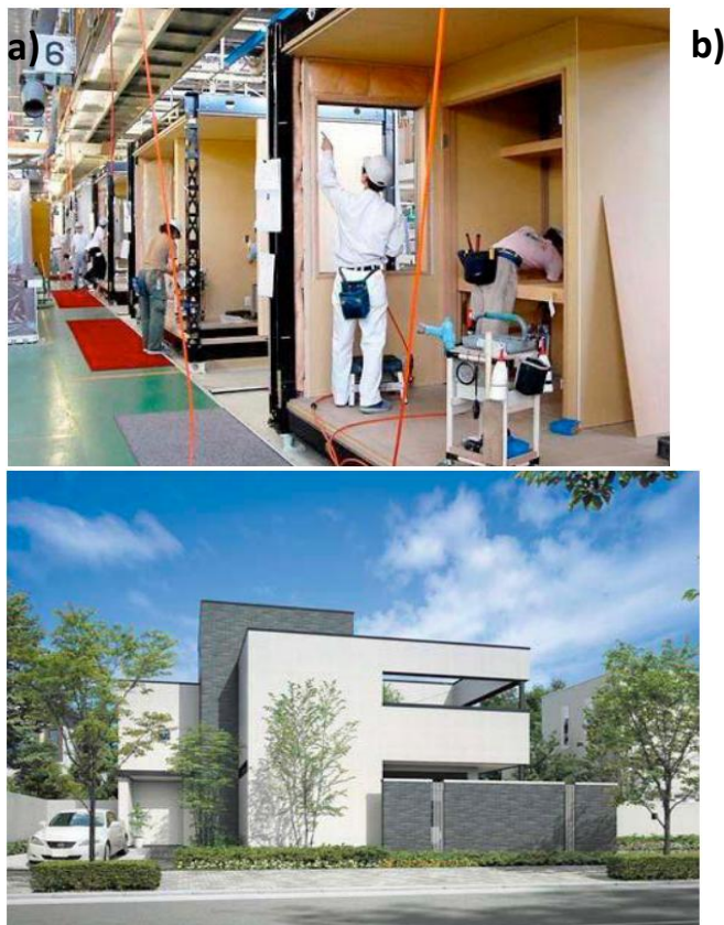
Figure 2 (a) Toyota Home Module fabrication at Toyota Home factory in Japan (b) Rendering of one of Toyota customizable home designs adopted from (Abulfahem, 2012)
