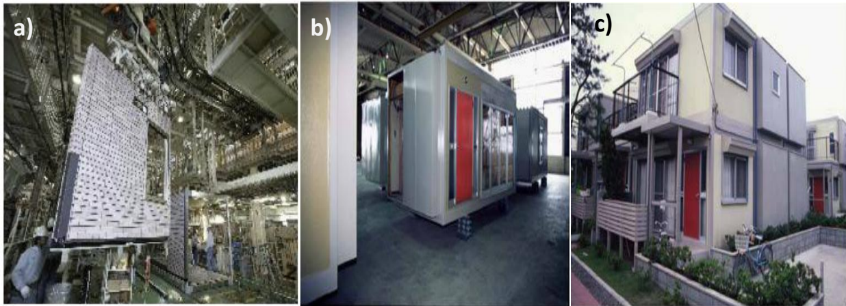
Figure 1 (a) Sekisui Heim wall elements production (b) Sekisui Heim Module (c) completed the installation of Sekisui house adopted from (Linner & Bock, 2012)
