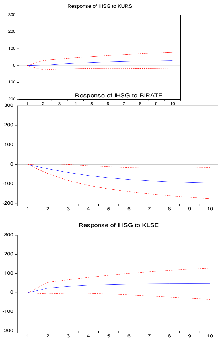
Figure 2 : Impulse Response Function (IRF) IHSG
