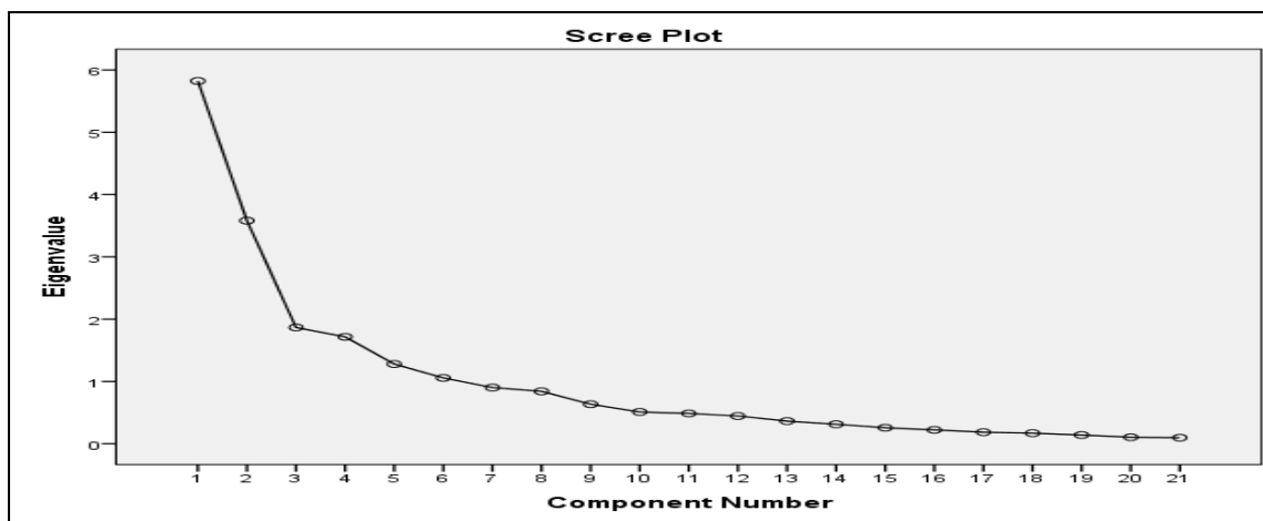
Figure 2: Scree plot
