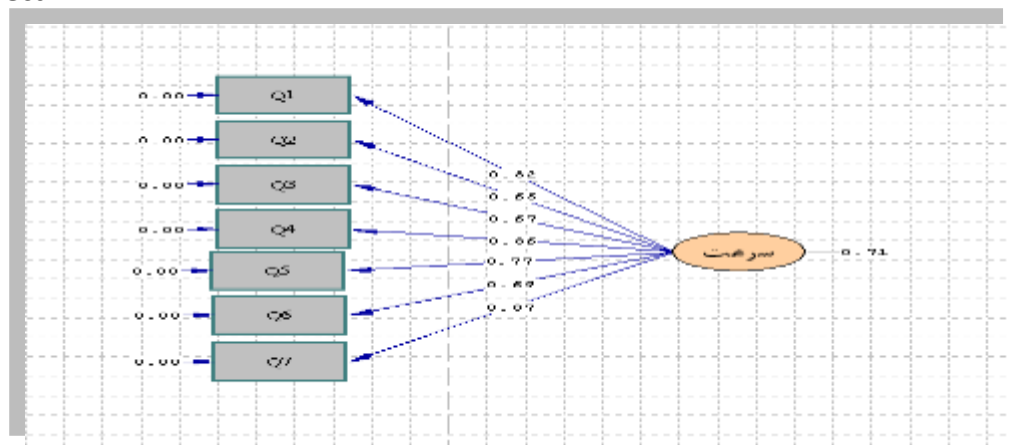
Diagram 1. Confirmatory factor analysis related to the speed index
