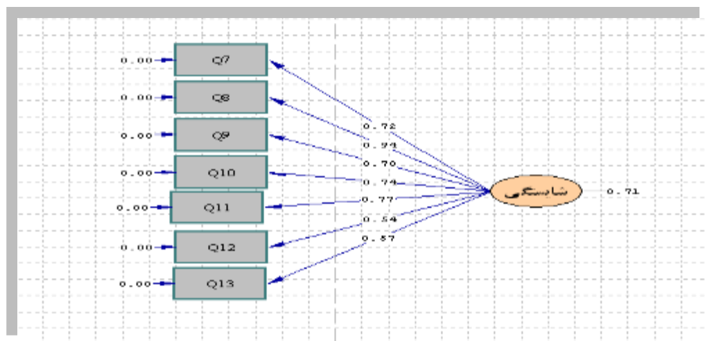
Diagram 2. Confirmatory factor analysis related to the competency index
