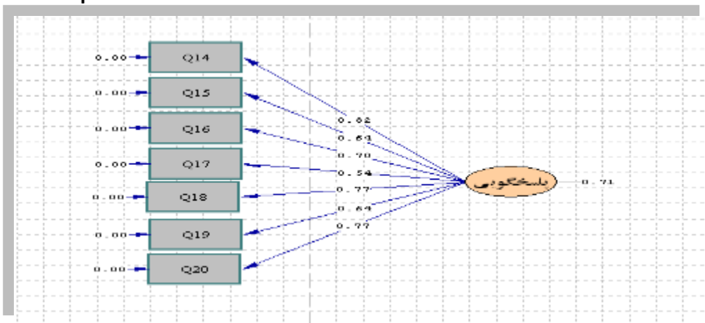
Diagram 3. Confirmatory factor analysis related to the responsiveness index
