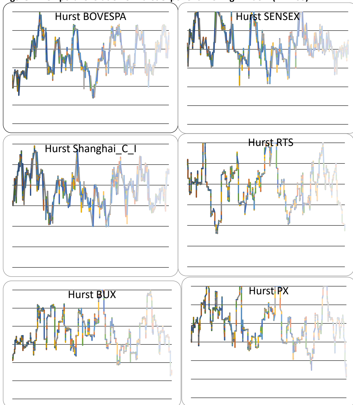
Figure 1. Temporal evolution of Hurst exponent - rolling window ( n = 100 )
