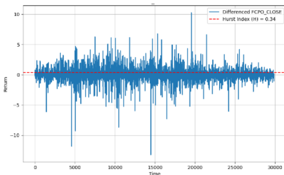
Figure 1.3 Differenced FCPO Price Series with Hurst Index
