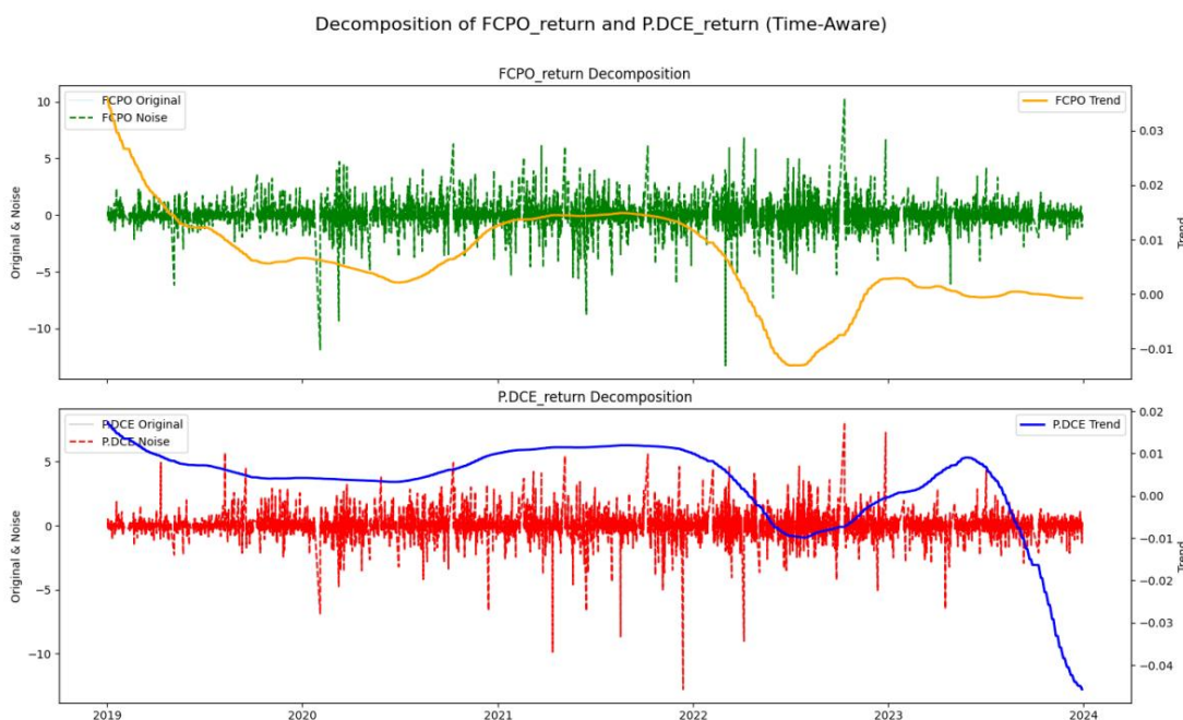
Figure 1.9 Trend and Noise Components of FCPO and P.DCE Returns
