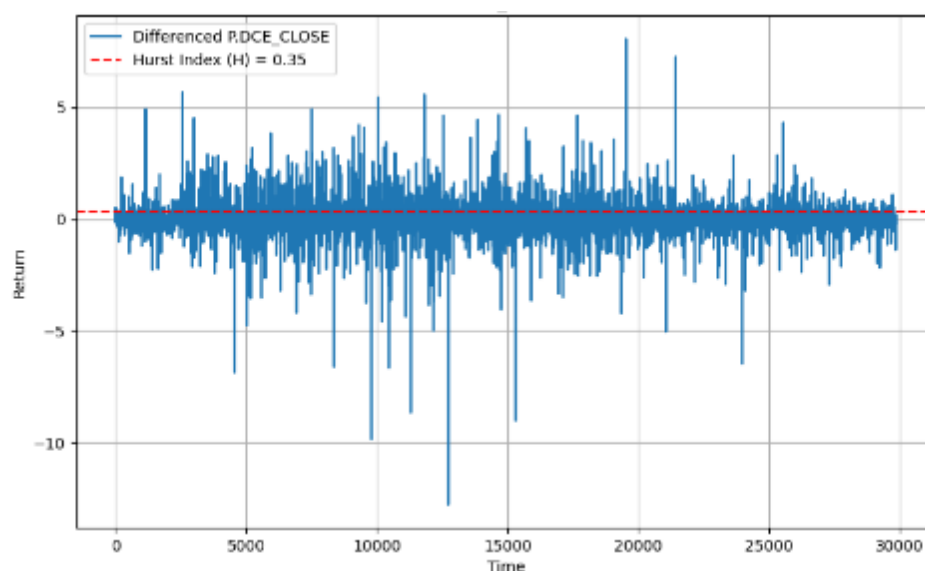
Figure 1.4 Differenced P.DCE Price Series with Hurst Index
