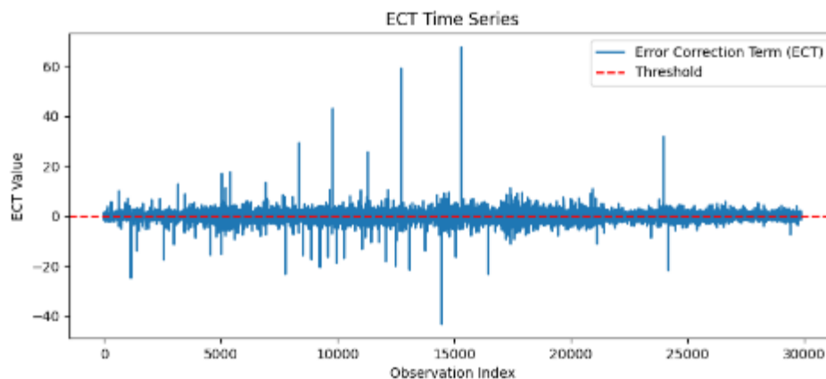
Figure 1.7 Asymmetric Adjustment Dynamics Around the Cointegration Equilibrium
