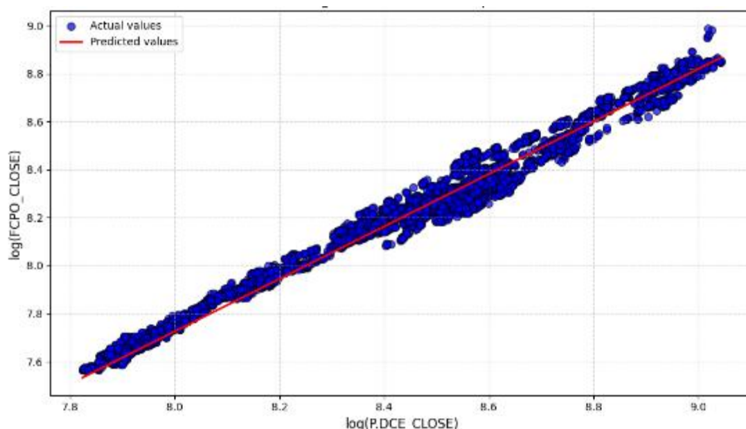
Figure 1.5 The Result of SVR with Linear Kernel Model
