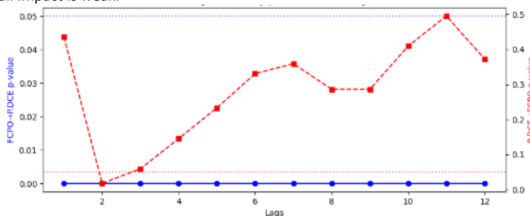
Figure 1.10 Conventional Granger Causality Test: p-values Across Different Lags [Source: The author]
