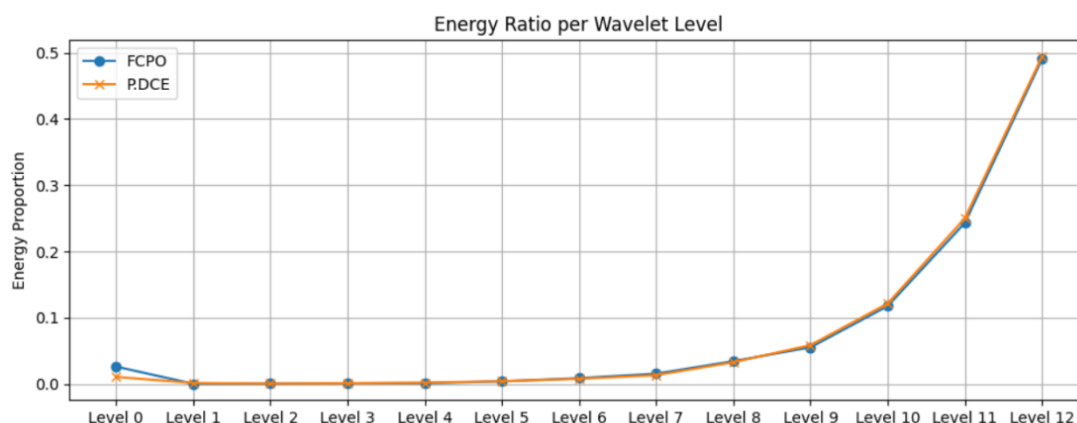
Figure 1.8 Wavelet Energy Distribution Between FCPO and P.DCE
