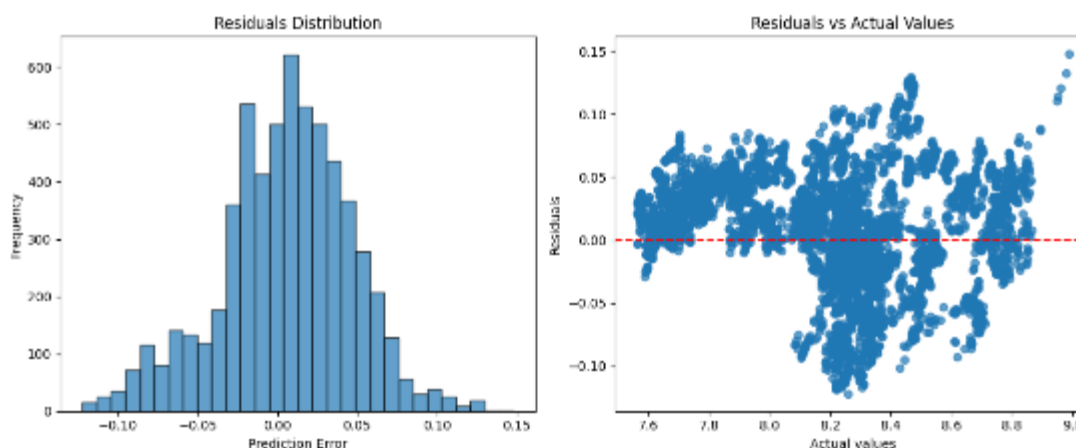
Figure 1.6 The Residual Analysis of SVR with Linear Kernel Model
