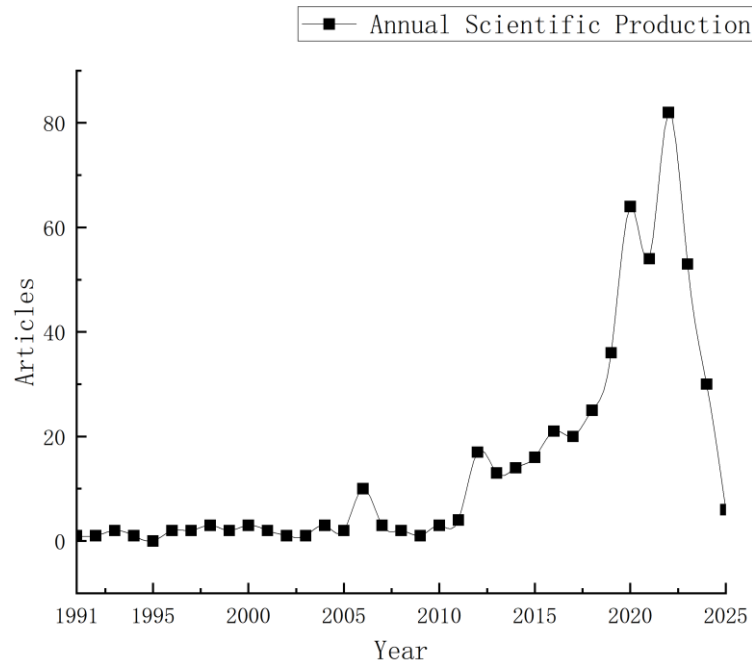
Figure 2. Annual Scientific Production for Ground Settlement Induced by Shield Tunnel Construction.
