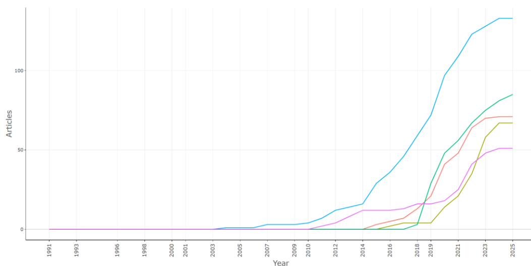
Figure 3. Affiliations' Production over Time for Ground Settlement Induced by Shield Tunnel Construction.
