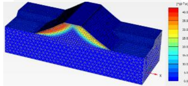
Figure 4. The FEM Model Slope
