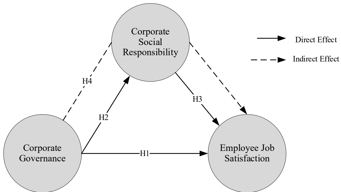
Figure 1. Theoretical model
