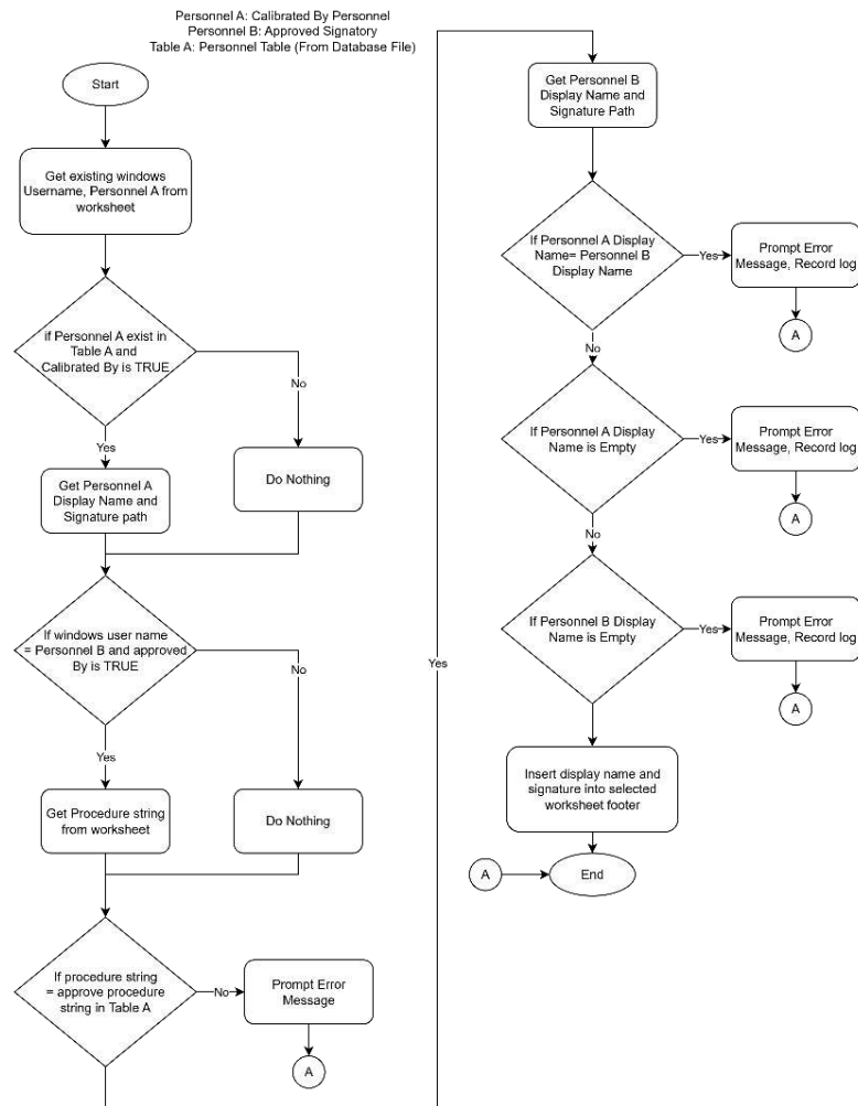
Figure 4.2 Approval process workflow
