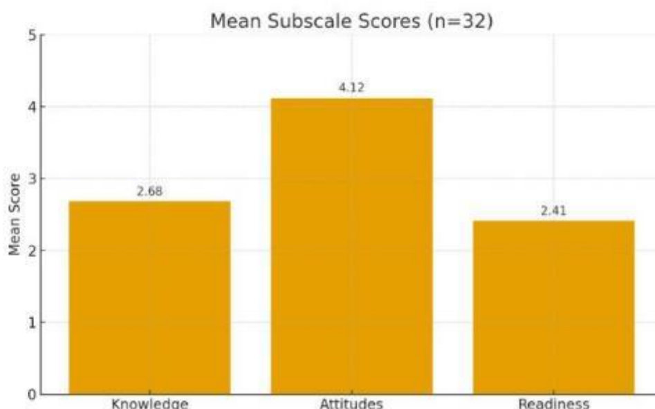
Figure 1: Subscale Means
