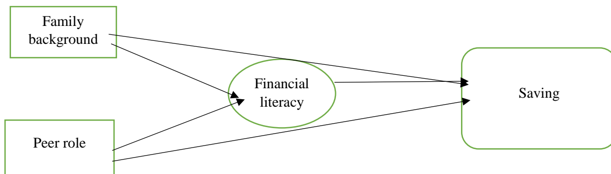
Figure 01: Framework
