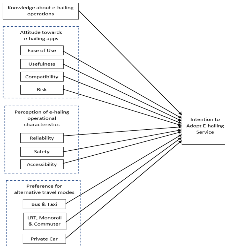
Figure 1: Research Framework
