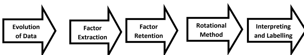
Figure 1. Exploratory Factor Analysis Implementation Stages
