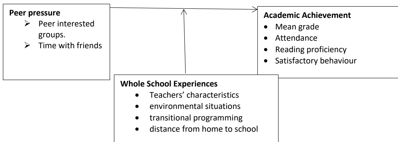
Figure 1.2 Conceptual Framework
