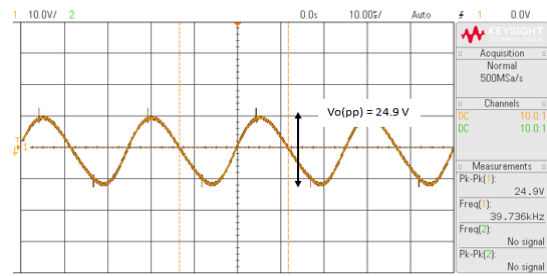
(b) The output voltage experimental result
