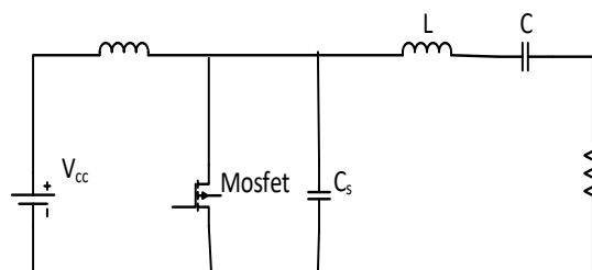
Figure 4: A single-ended Class E ZVS inverter (Kazimierczuk, 2014),
