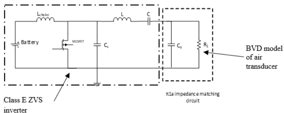
Figure 15: Suggested Class E ZVS inverter with \pi 1a matching network for future design
