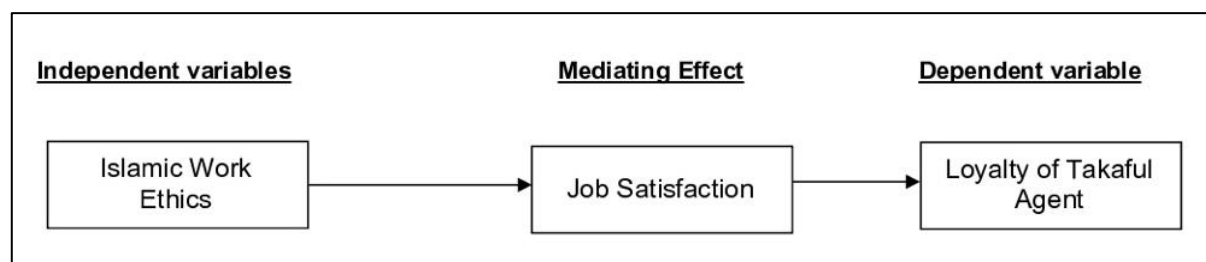
Figure 4.2.1 Theoretical Framework
