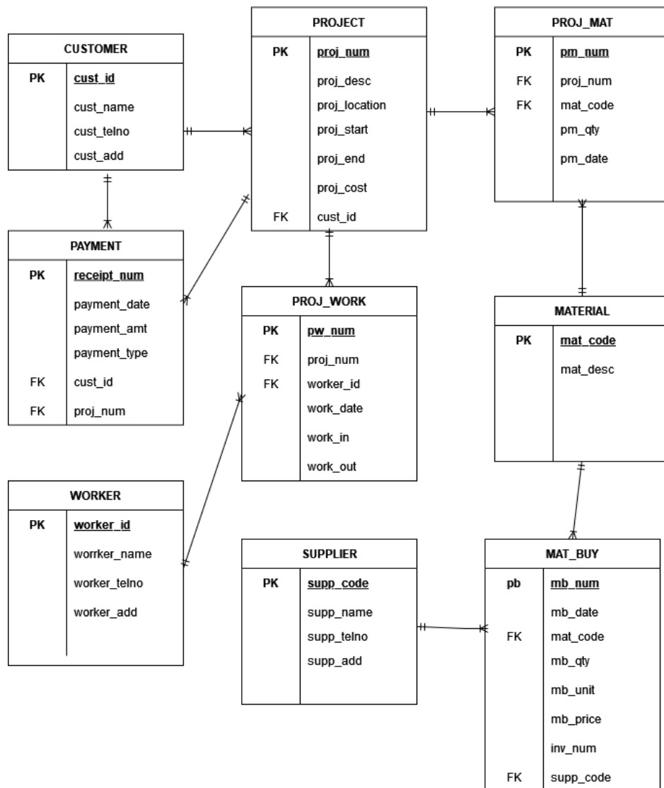
Figure 11: Database conceptual diagram for SME Construction Business
