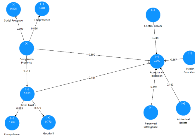
Figure 3: Measurement model assessment
